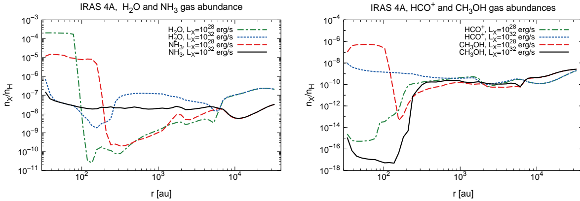
Fig. 1. [Left panels]: The green dashed dotted line and the blue dotted line show radial profiles of \text{H}_2\text{O} gas fractional abundances with respect to total hydrogen densities ( n_{\text{H}_2\text{O}}/n_{\text{H}} ) for values of central star X-ray luminosities L_X=10^{28} and 10^{32} \text{erg s}^{-1} , respectively. The red dashed line and the black solid line show radial profiles of \text{NH}_3 gas fractional abundances ( n_{\text{NH}_3}/n_{\text{H}} ). [Right panel]: The green dashed dotted line and the blue dotted line show radial profiles of \text{HCO}^+ gas fractional abundances with respect to total hydrogen densities ( n_{\text{HCO}^+}/n_{\text{H}} ). The red dashed line and the black solid line show radial profiles of \text{CH}_3\text{OH} gas fractional abundances ( n_{\text{CH}_3\text{OH}}/n_{\text{H}} ). In this Figure, these profiles are based on calculations of NGC 1333-IRAS 4A envelope models in Notsu et al. (2021).
